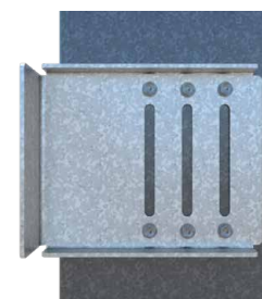
12ga Clip: (6) #12-14 Screws 14ga Clip: (6) #10-16 Screws Shown in a UBC6 Clip
