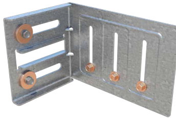
STRUCTURE AND FRAMING OFFSET CONNECTION 2 Drift Bushings & Framing Fasteners
