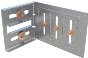
STRUCTURE AND FRAMING CENTERED CONNECTION 1 Drift Bushings & Framing Fasteners
