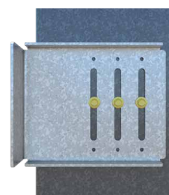
(3) #14 Deflection Screw Pattern Shown in a UBC6 Clip
