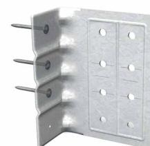
Location Options with (3) Anchors
