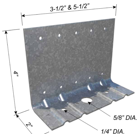
EasyClip T-Series Tall Anchor Clip
