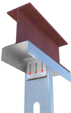
FRAMING OFFSET CONNECTION
