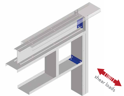
Head-to-Jamb Connections
